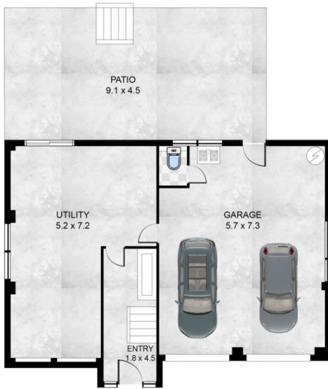
FLOOR 1
